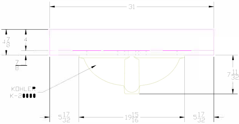
FRONT VIEW
