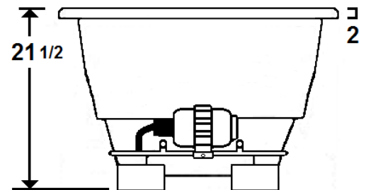
Standard (S) Blower & Heater Location
