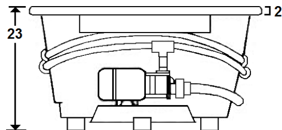
Standard (S) Silent Pump w/ Heater Location
