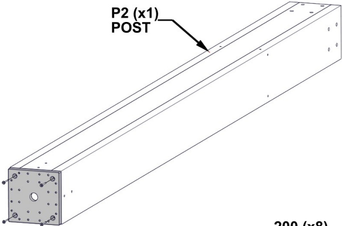
200 (x8) SCREW - 1 1/2"
