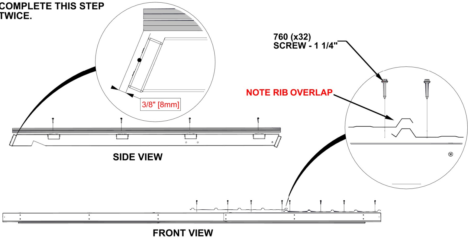
125 (x2) 29 GA STEEL SHEETING
