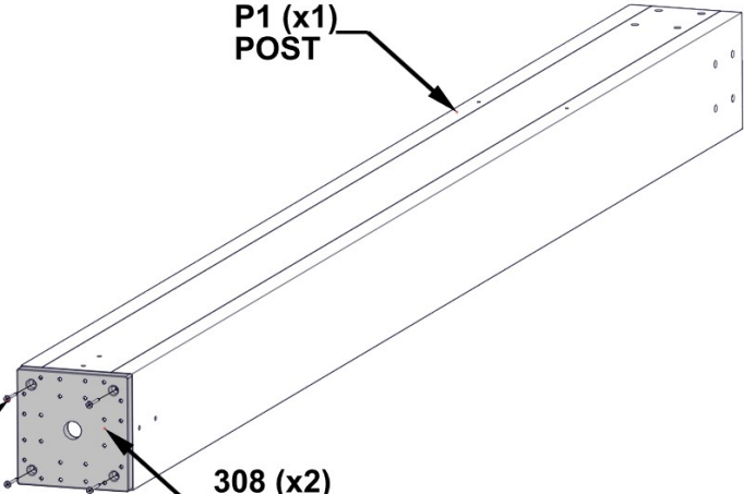
308 (x2) 6x6 POST FOOT
