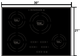
Cooktop Dimensions
