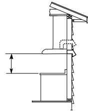
Wall Venting
