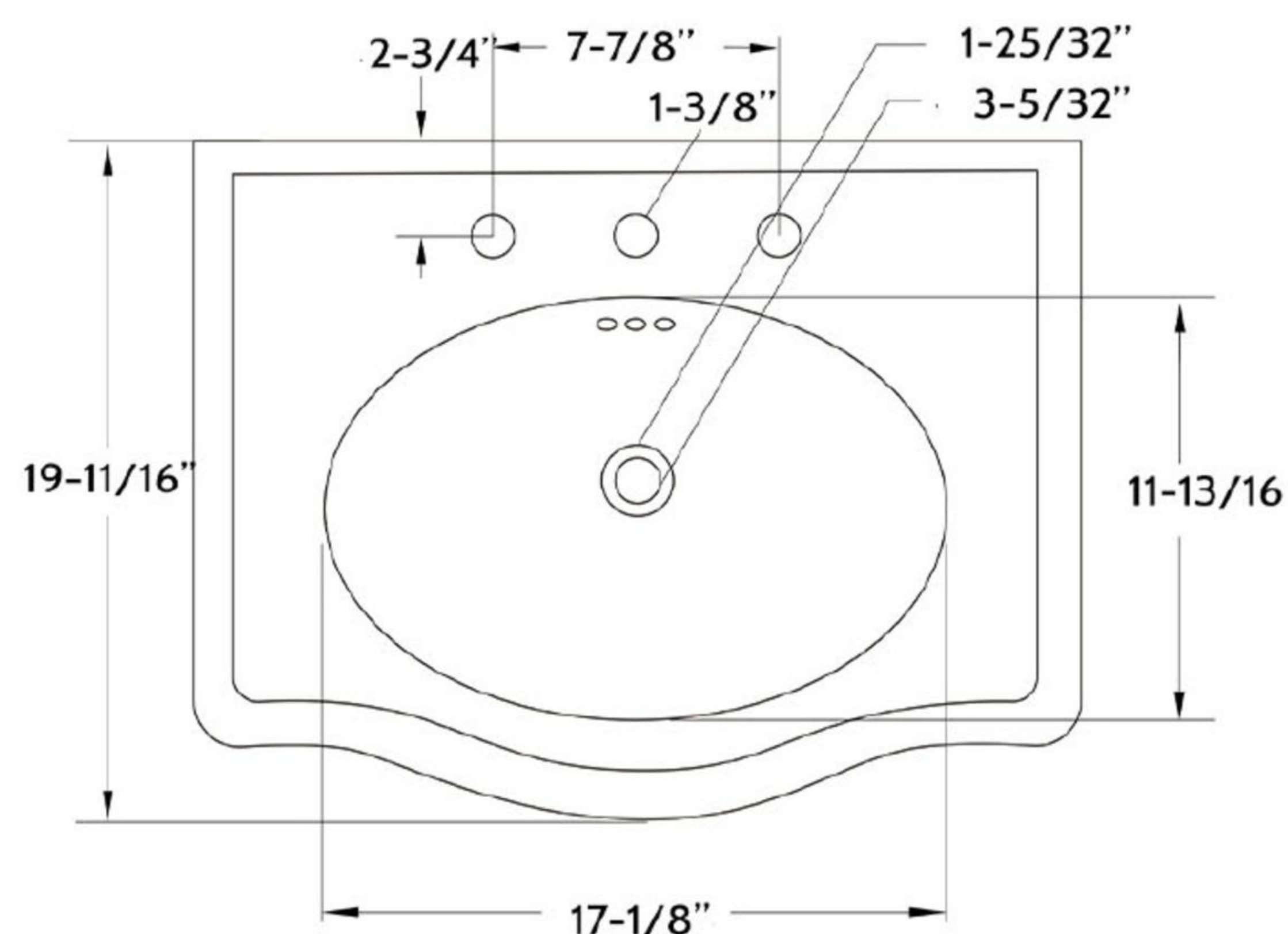
TOP VIEW
