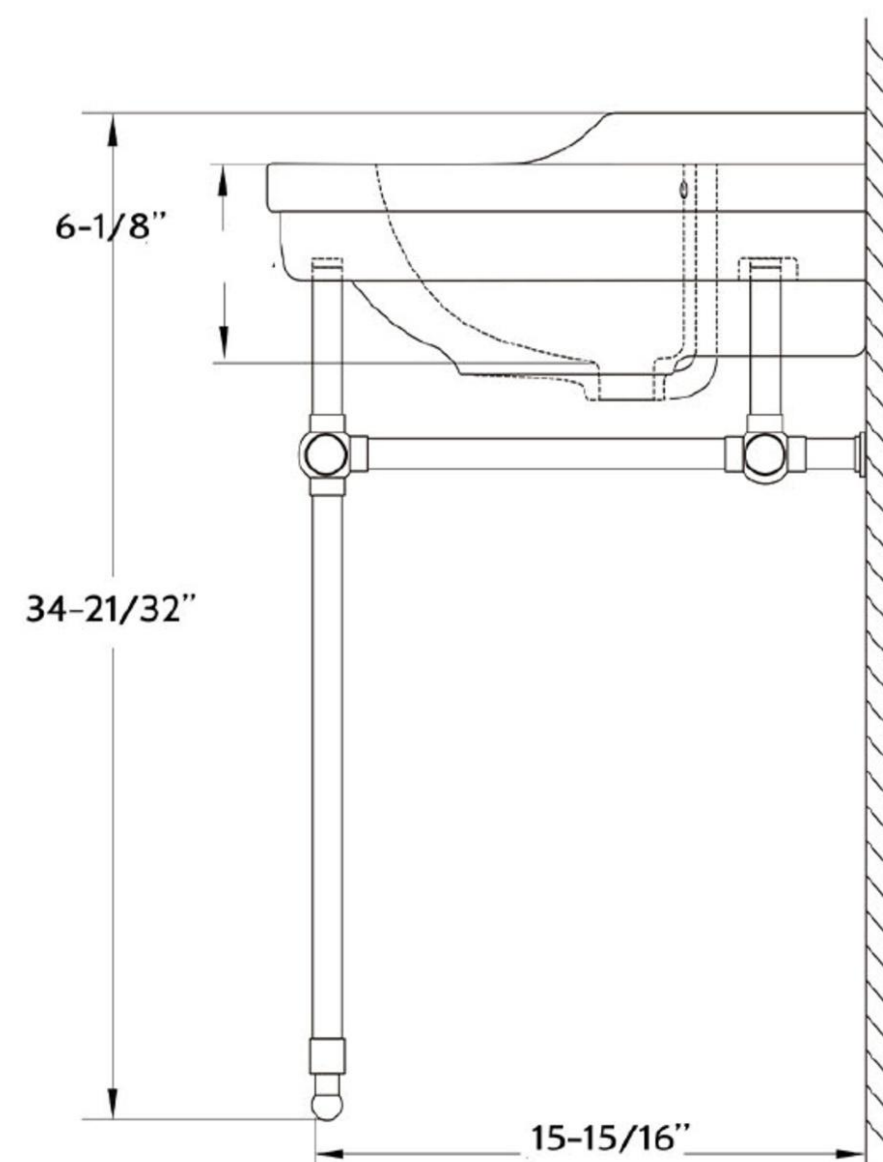
SIDE VIEW
