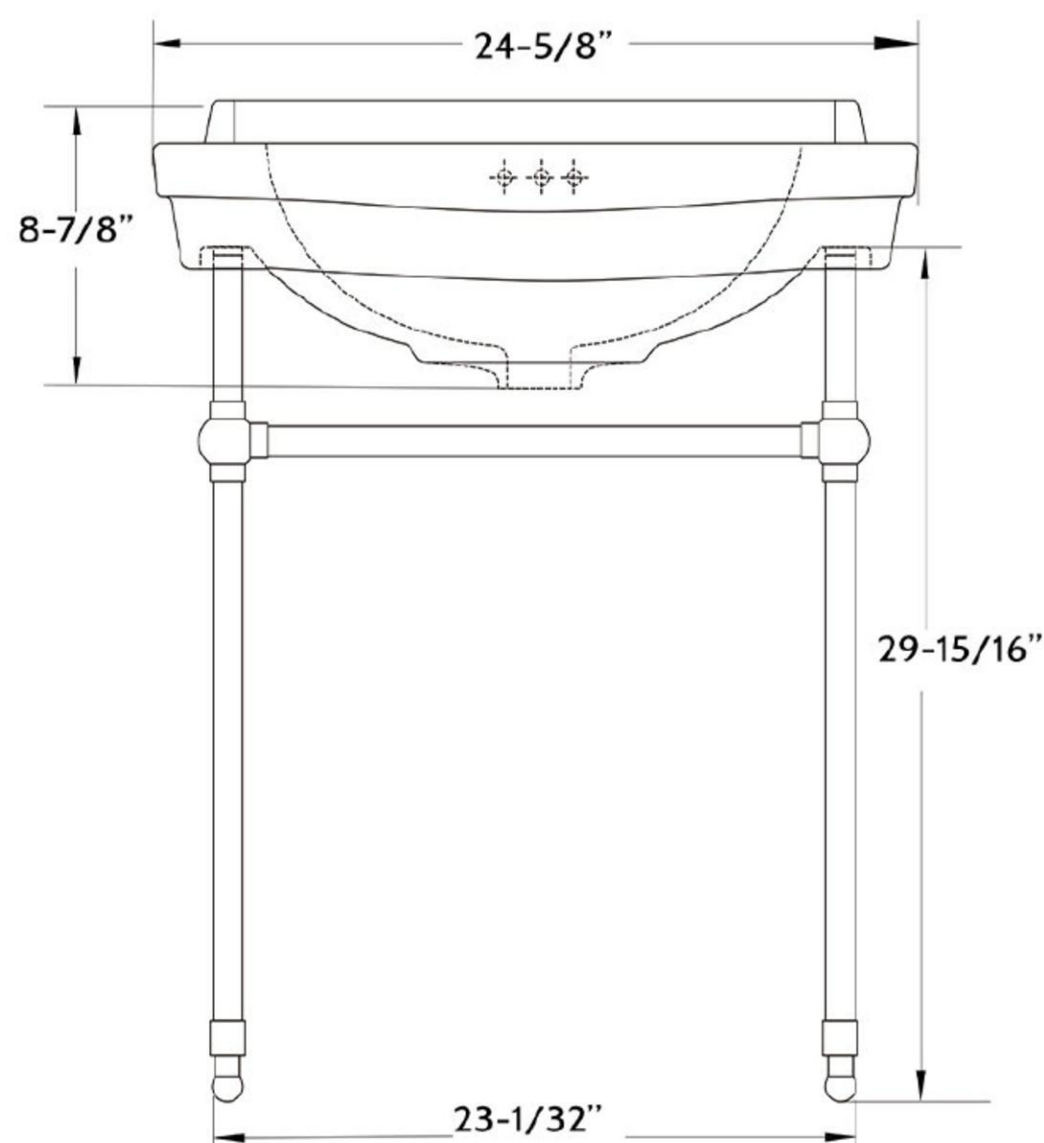
FRONT VIEW
