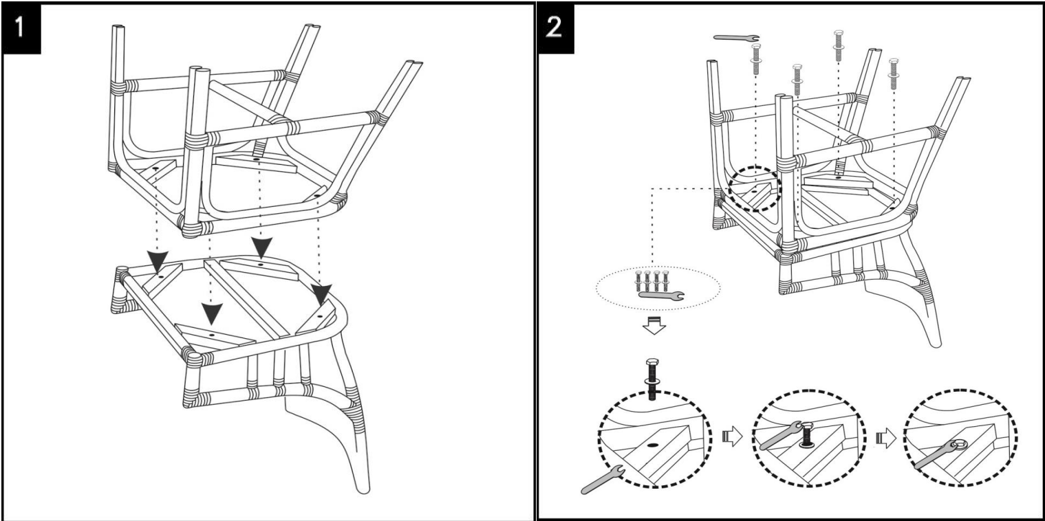
Assembly part A and B with Nuts and tighten with Pass key
