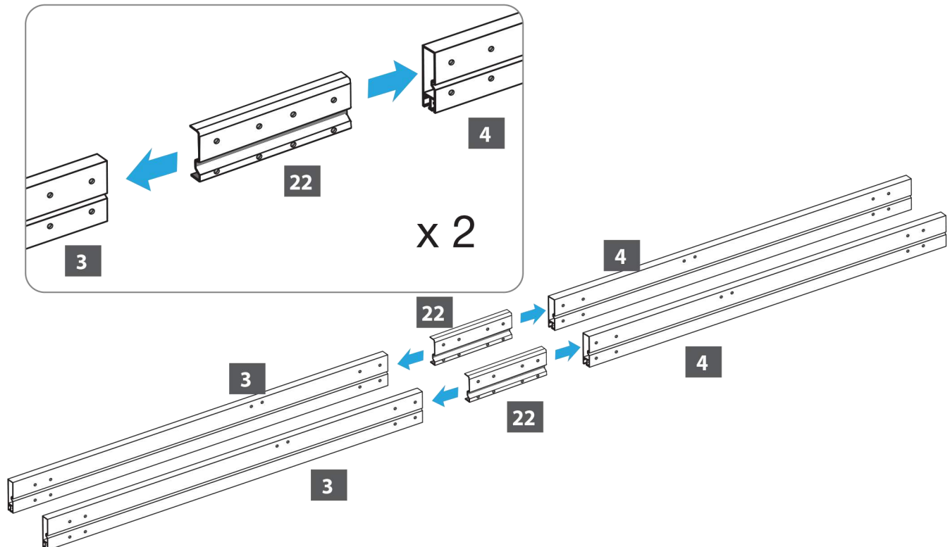
Roof profile (3) 1822mm x 2
