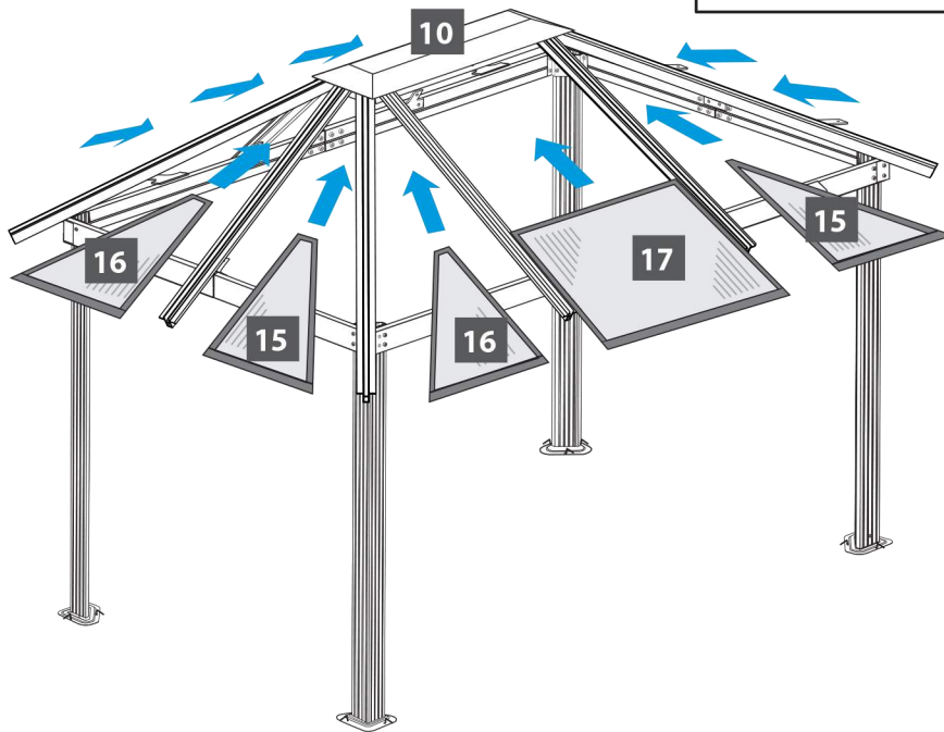
Roof panel (15) x 4
