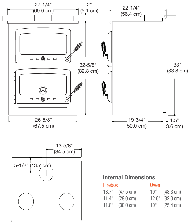
Figure 9 Dimensions for installer
