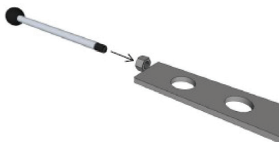
Figure 2 Top air control rod installation
