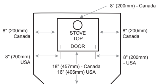
Figure 3 Non-combustible floor protector requirements
