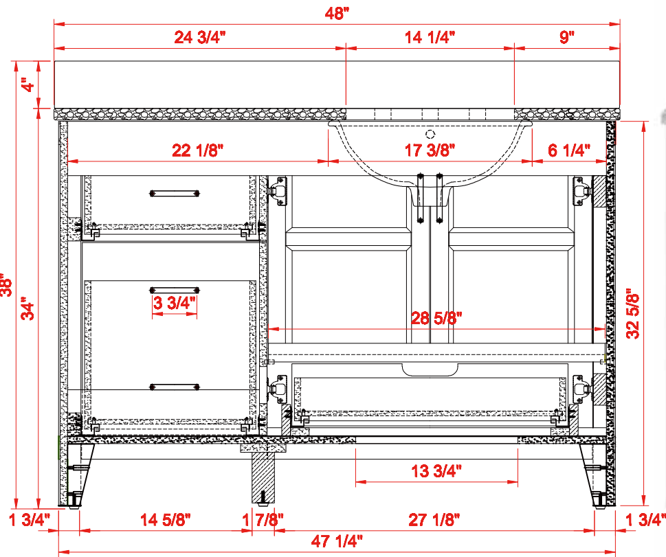
BACK VIEW
