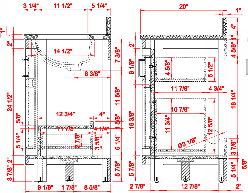
SIDE VIEW
