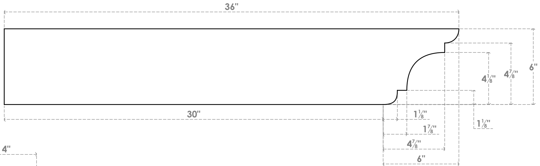
SIDE PROFILE
