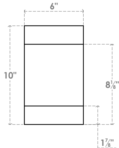
FRONT PROFILE
