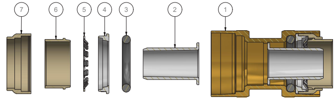
Exploded View
