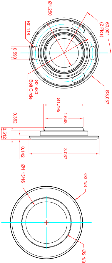
IFSS-CER-FLANGE Detail
