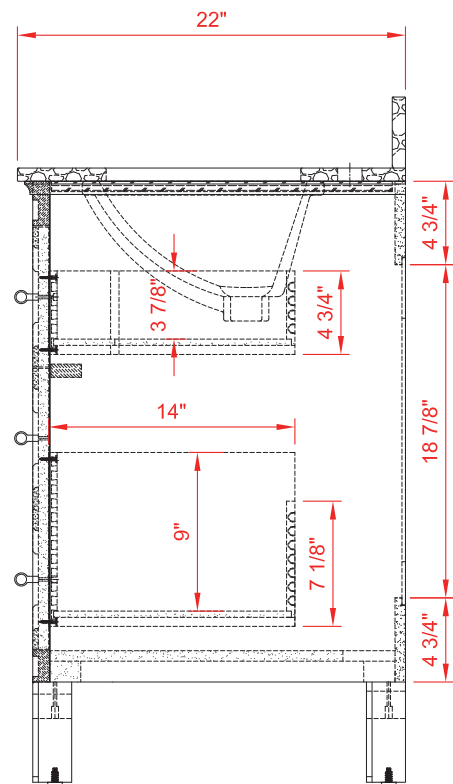
SIDE VIEW
