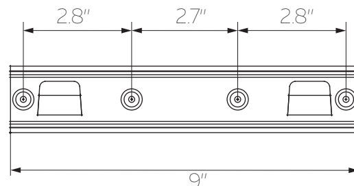
LOWER BRACKET
