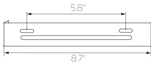
UPPER BRACKET
