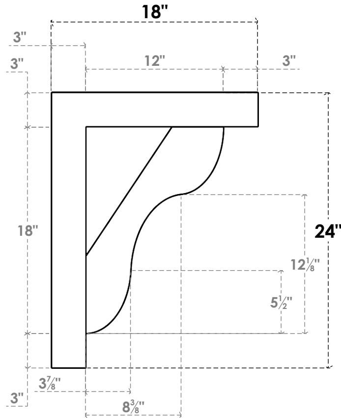
SIDE PROFILE
