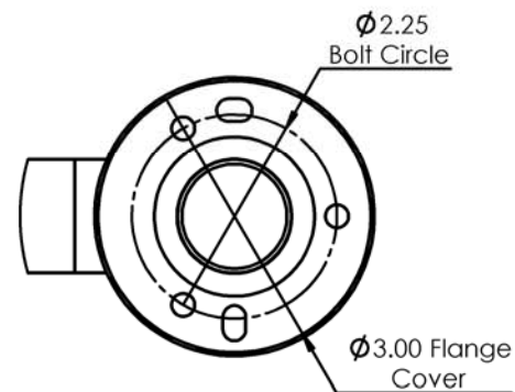
Flange Detail A
