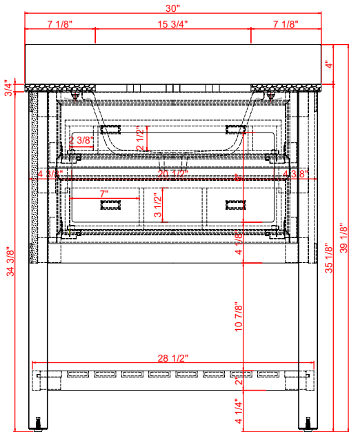
BACK VIEW
