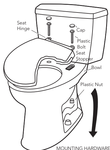
MOUNTING HARDWARE
