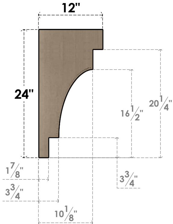
SIDE PROFILE
