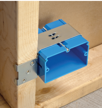
Clip the Adjust-A-Box® metal bracket onto the stud for square, secure mounting.
