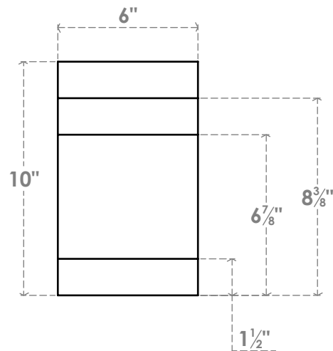
FRONT PROFILE
