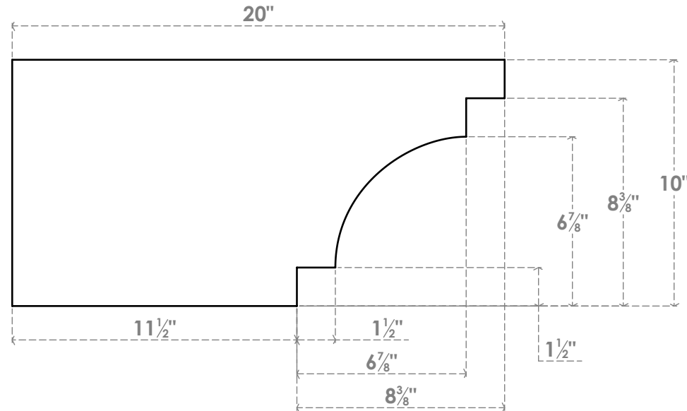
SIDE PROFILE
