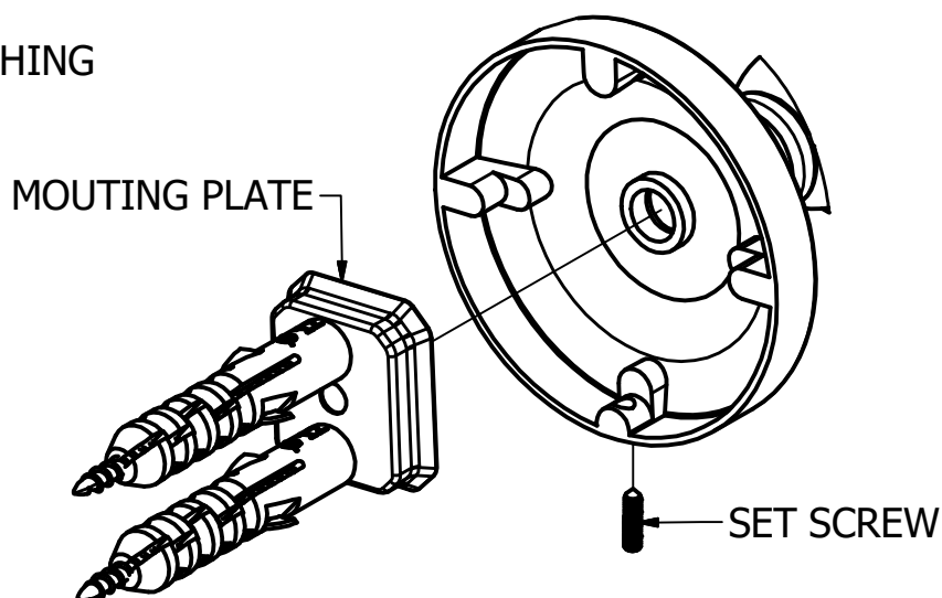
DETAIL D
