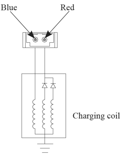
(Charging Diagram)
