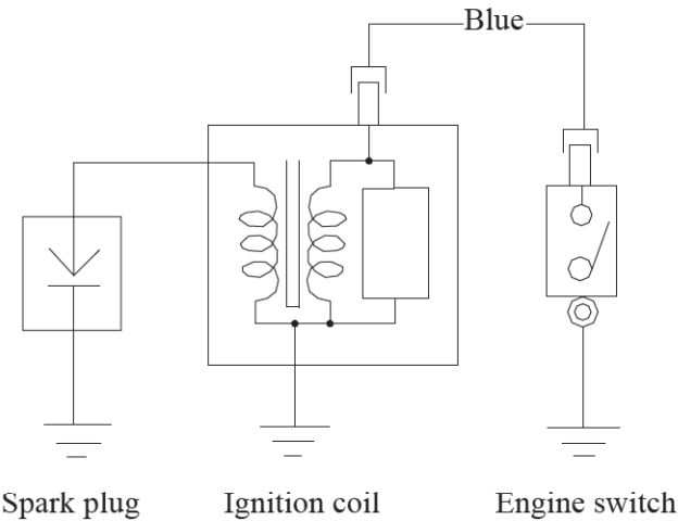
(Ignition System Circuit Diagram)
