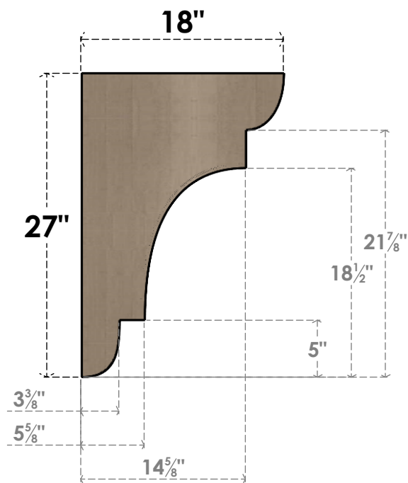
SIDE PROFILE
