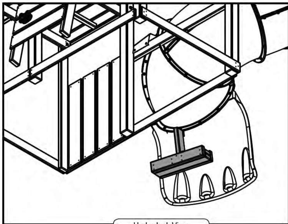
Underdeck View
