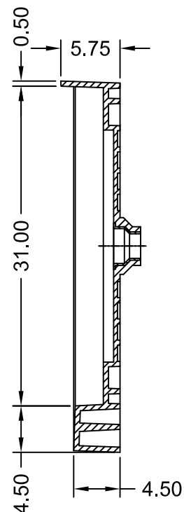
SECTION B-B
