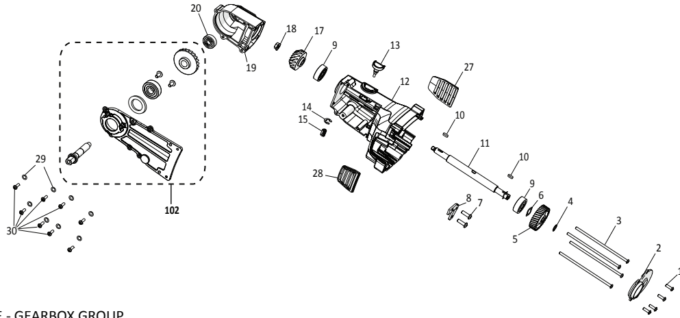
E - GEARBOX GROUP
