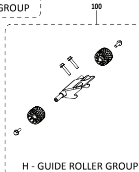
H - GUIDE ROLLER GROUP
