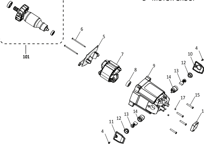
D - MOTOR GROUP
