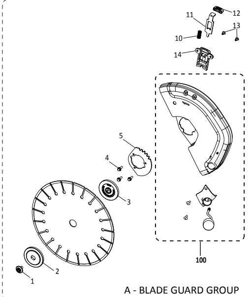
A - BLADE GUARD GROUP
