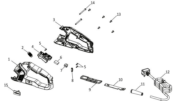
C - REAR HANDLE GROUP
