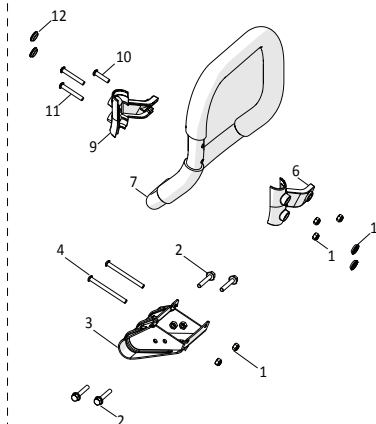
B - FRONT HANDLE GROUP
