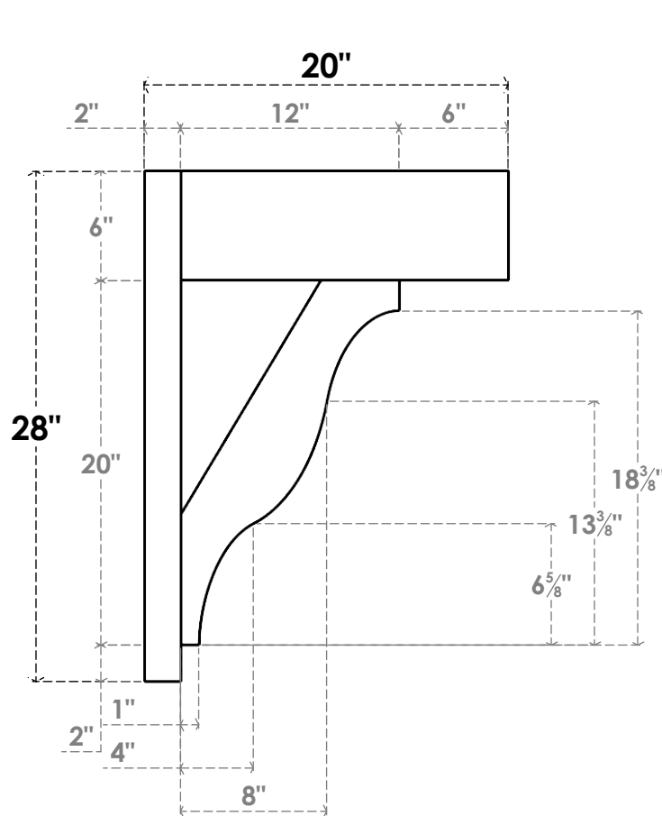
SIDE PROFILE
