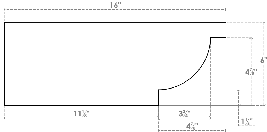
SIDE PROFILE
