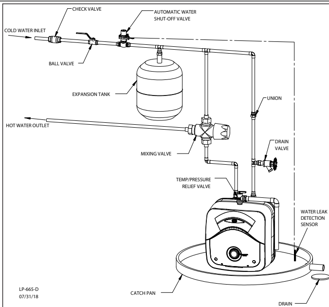
Figure 2 - Installation Detail
