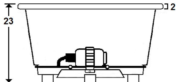
Standard (S) Pump & Heater Location
