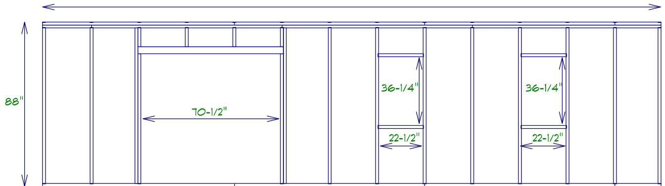
Front Wall Layout (Doors aligned to the left) 26'
