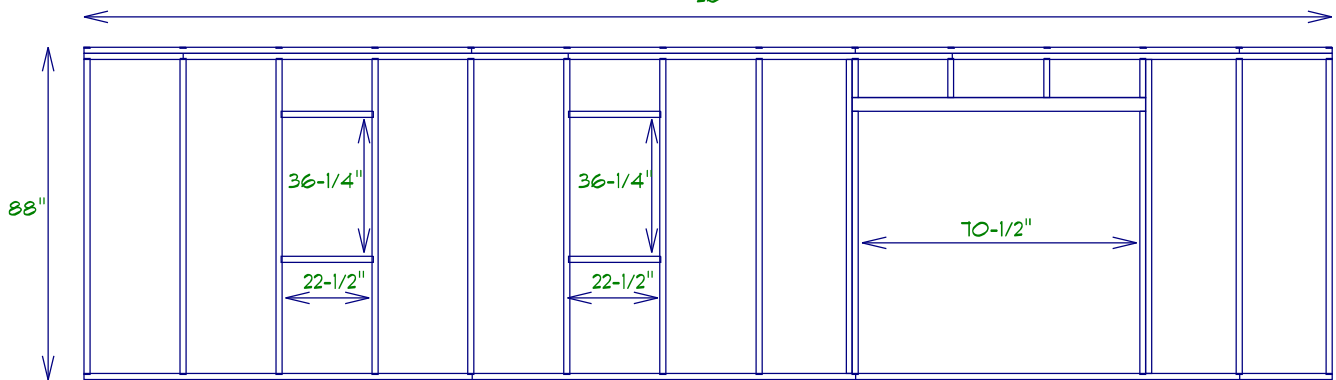
Front Wall Layout (Doors aligned to the right.)
