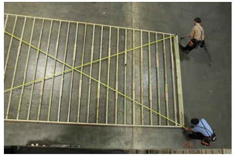
(21) Knock the joists on the end accordingly, till measurements are equal.
