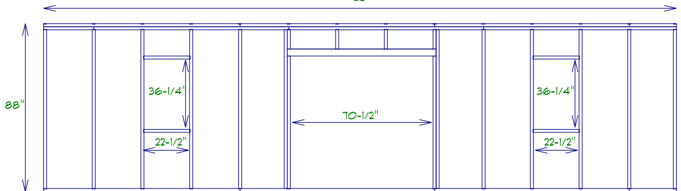
Front Wall Layout (Doors aligned to the center) 26'
