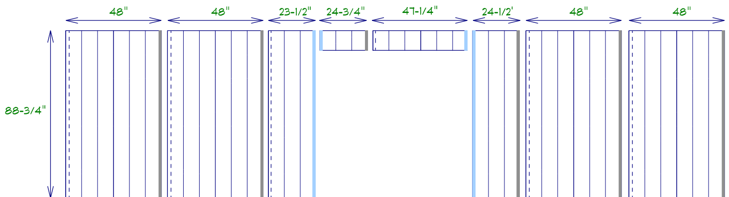
Front Wall Siding Layout (Doors aligned to the center)
