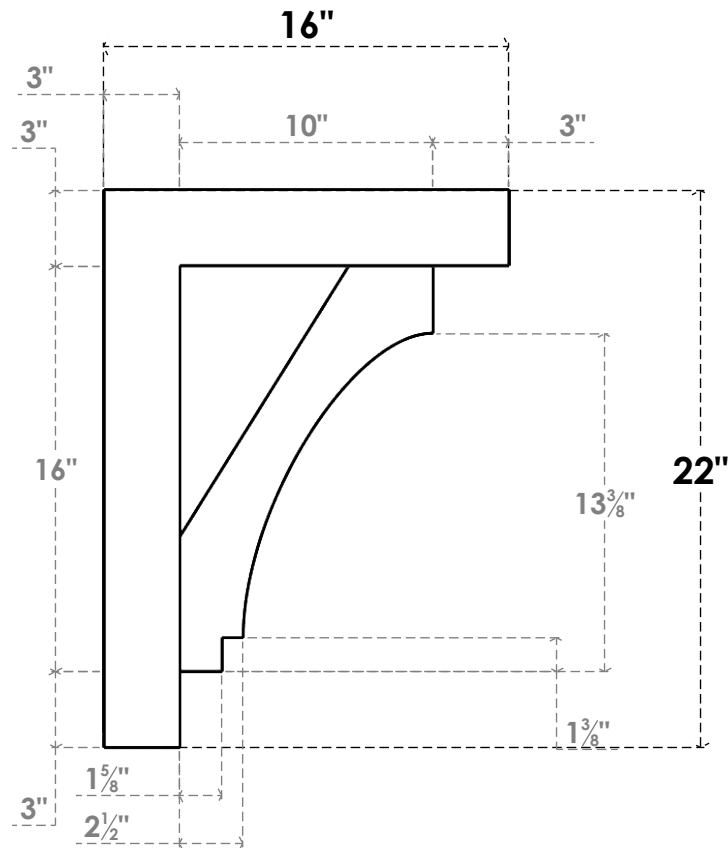
SIDE PROFILE
