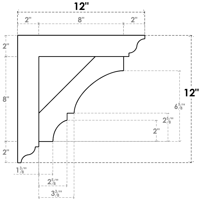
SIDE PROFILE
