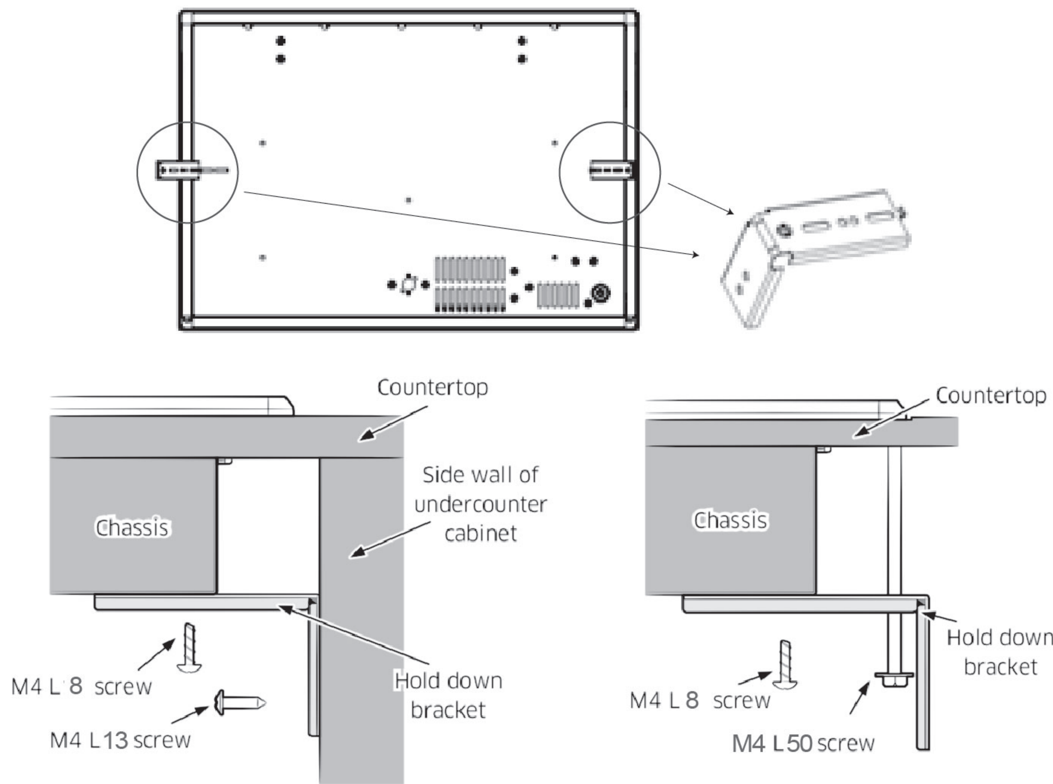
Installation Method 1
