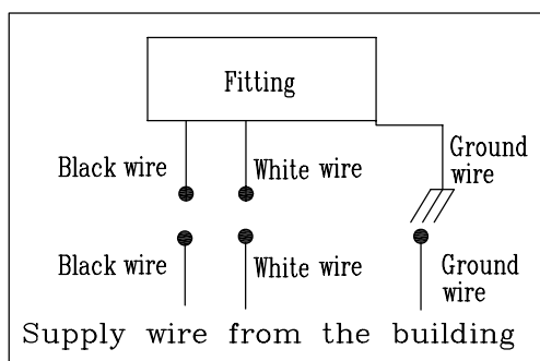
Circuit diagram 1
