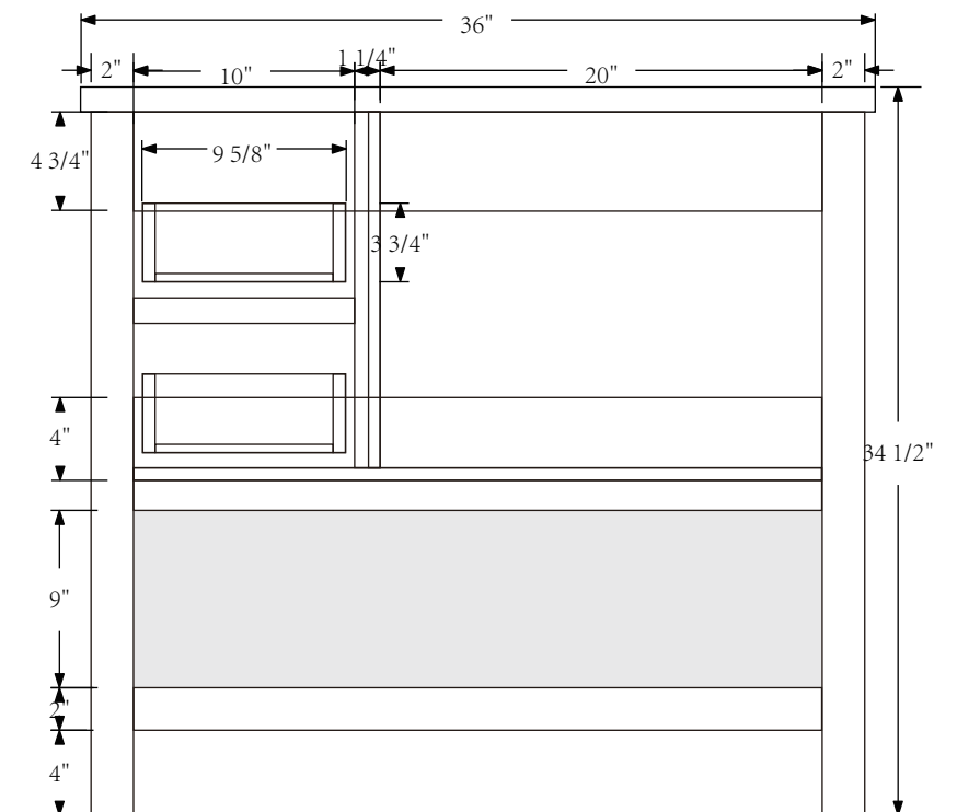
BACK VIEW
