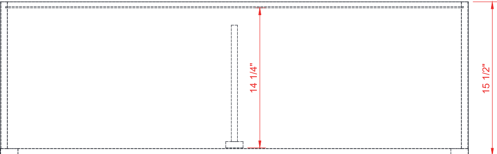
TOP VIEW
