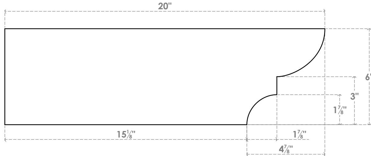
SIDE PROFILE
