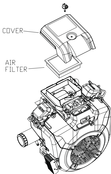
Figure 15 – Air Filter
