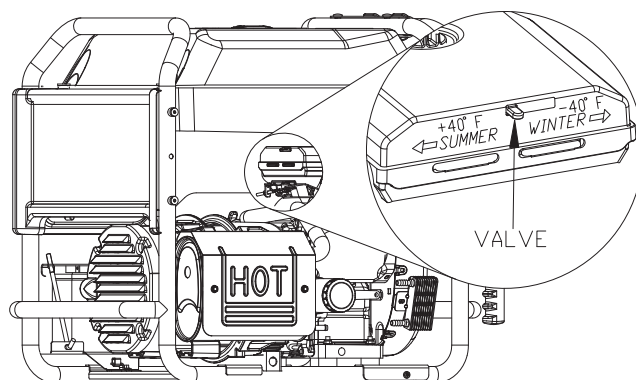
Figure 11 – Winter/Summer Valve
