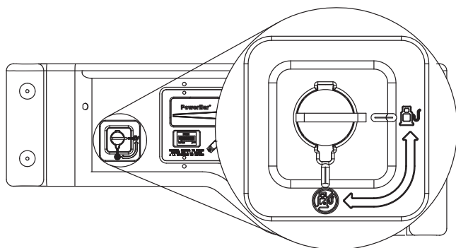
Figure 13 – Choke Operation
