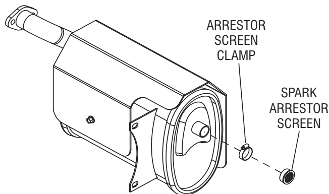
Figure 16 – Spark Arrestor Screen
