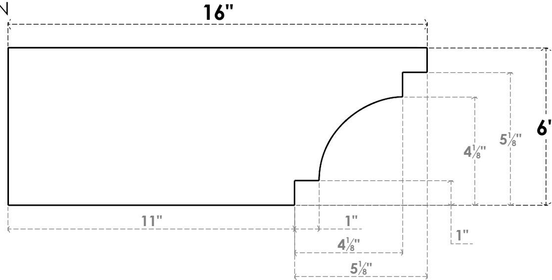
SIDE PROFILE
