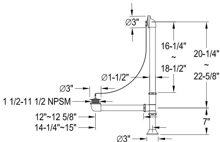
CC2091,2,5,8 Tub Waste & Overflow
