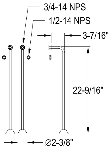
CC461,2,5,8 Single Offset Bath Supply
