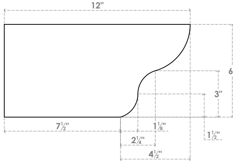
SIDE PROFILE
