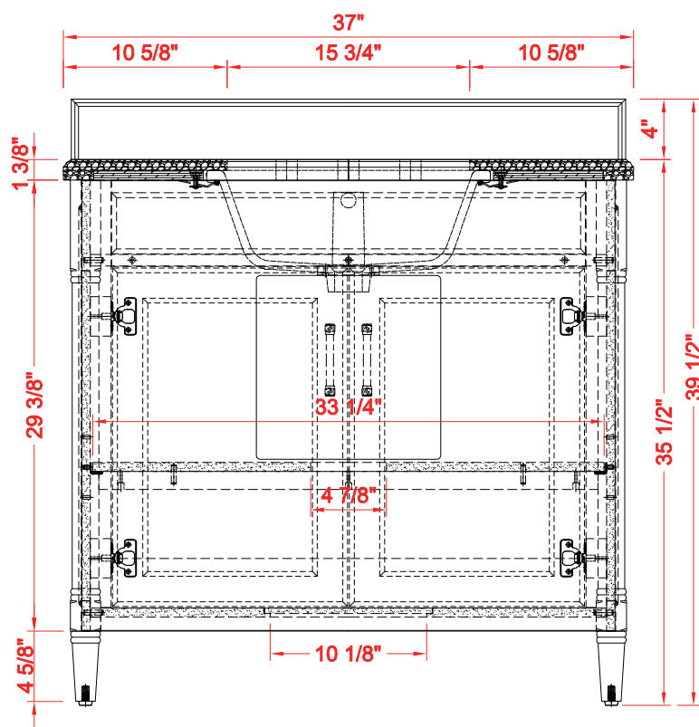
BACK VIEW
