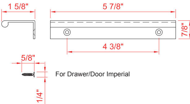
HANDLE
