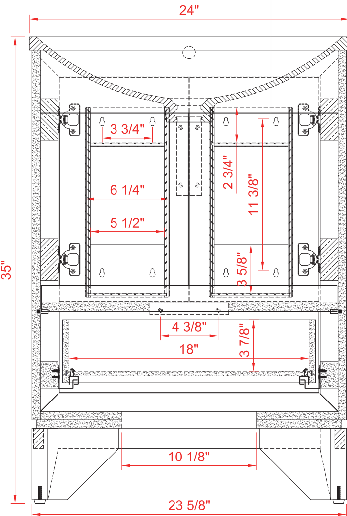
BACK VIEW
