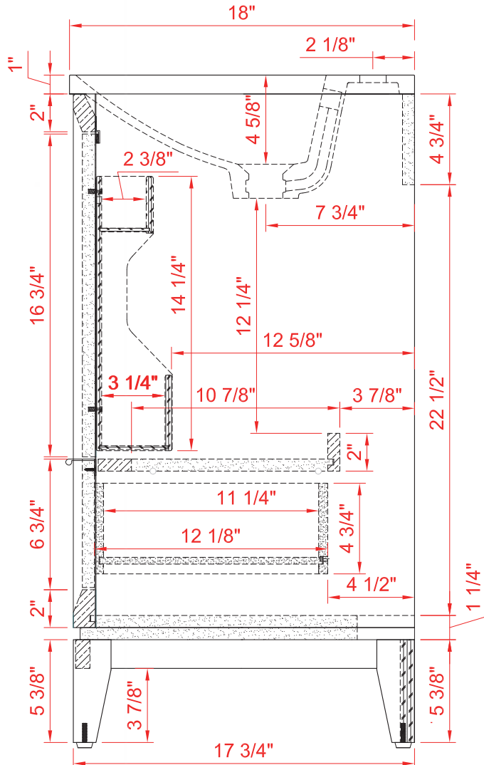
SIDE VIEW
