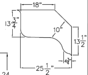
SEAT DIMENSIONS
