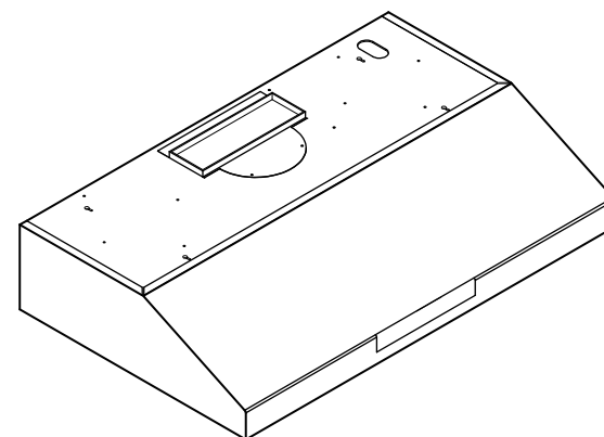
TOP RECTANGULAR EXHAUST ADAPTER
